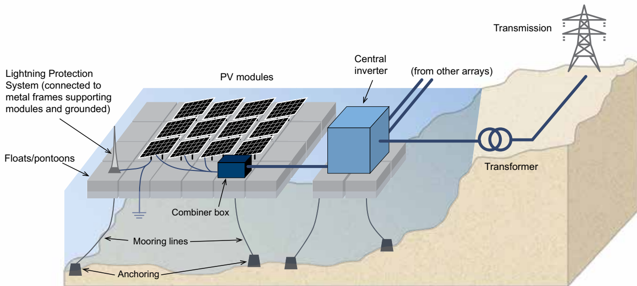
FIGURE 1 Schematic representation of a typical large-scale floating PV system with its key components
