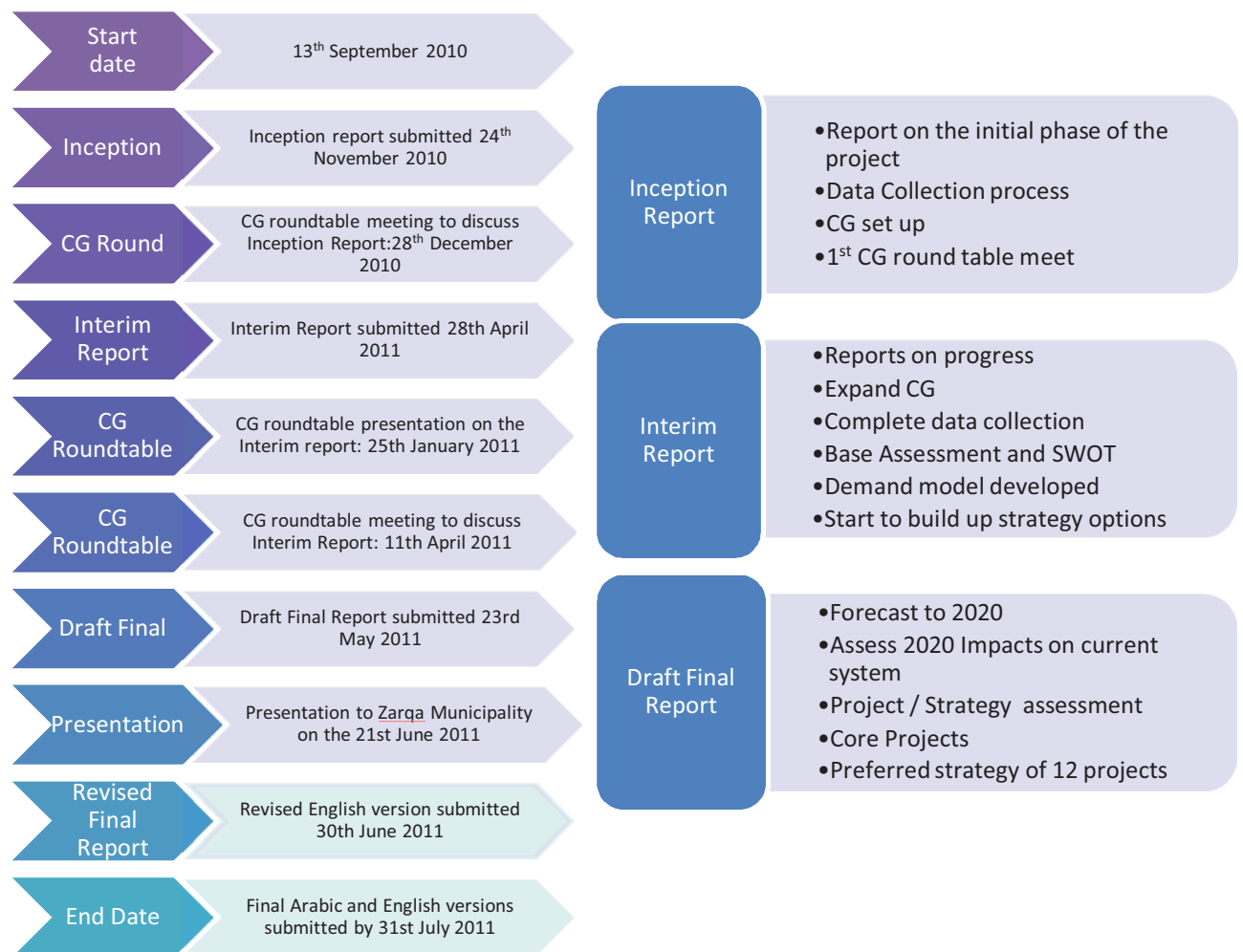
Figure 2.1: Work Programme
